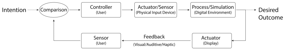
Figure 29.1. Closed-loop control (real-time interactive) system for avatar control. (Source: author, adapted from Dorf & Bishop, 1998; Englander & Englander, 2003)
