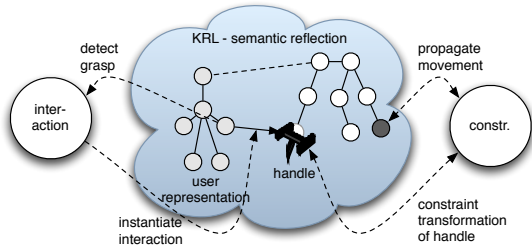
Figure 8: Interaction and constraint module (see text).
