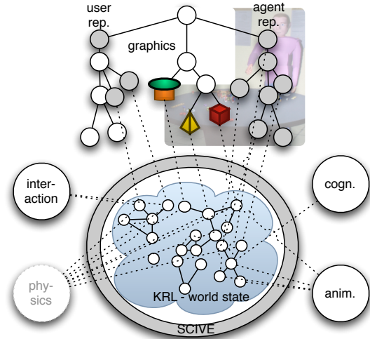
Figure 5: Application layout 2: SCIVE's KRL centered interconnection of user interaction, agent perception, animation, and physics modules (see text).
