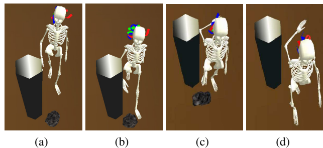
Figure 7: The animated agent filter in action. The motion captured animated agent collides with a relatively heavy (the column) and a lighter (the stone) obstacle in its pre-determined path. The collision signals the activation of an animation blending filter which controls the colliding body parts for the specific time interval whereas the collision objects stay under physics control.
